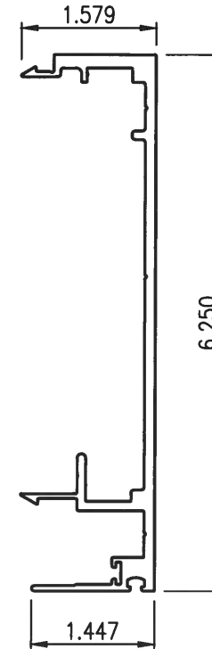
22 SUN-8110 SPLIT MULLION Scale: 6" = 1'-0"
