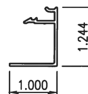
16 SUN-6290 SILL CLOSURE Scale: 6" = 1'-0"
