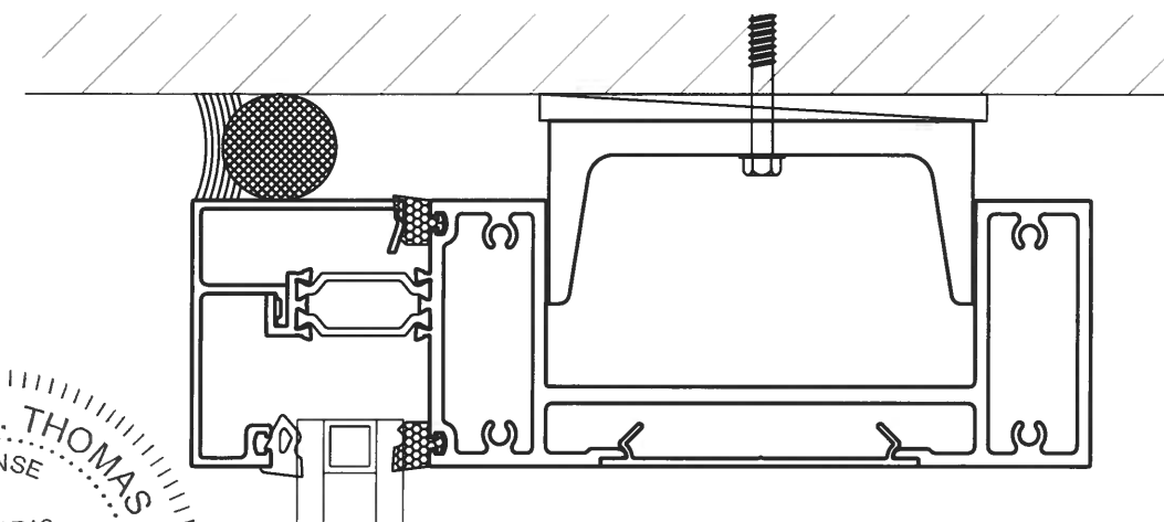
HEAD ANCHOR CONDITION A (CHANNEL) REF DETAIL 4 ON SHT 4
