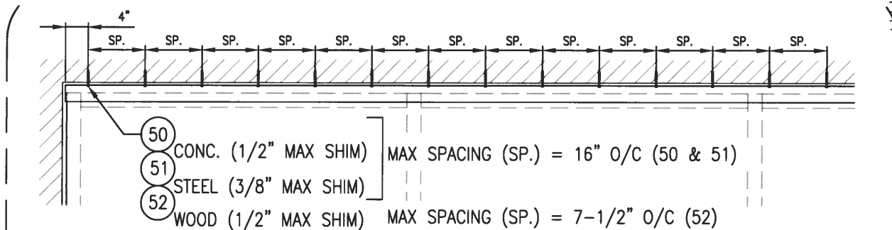
HEAD RECEPTOR (CONDITION B)
