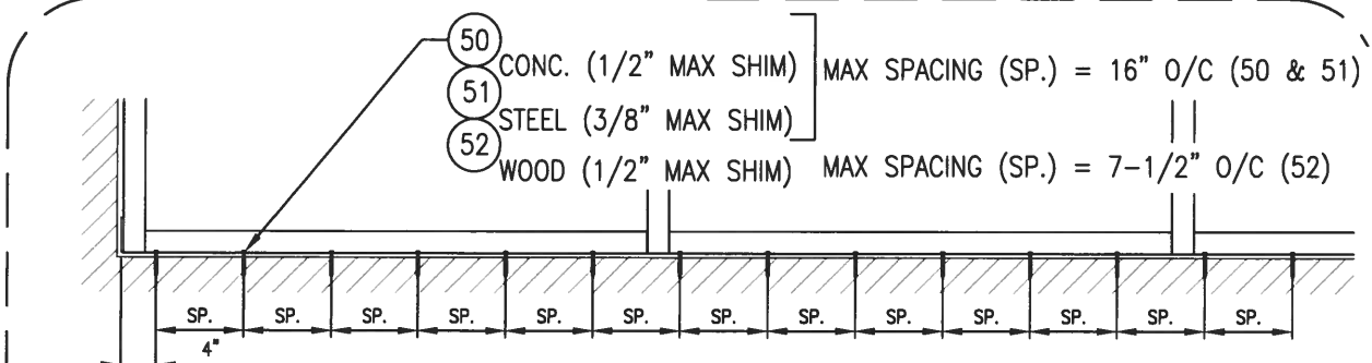
SILL ANCHOR SPACING (ALL CONDITIONS)
