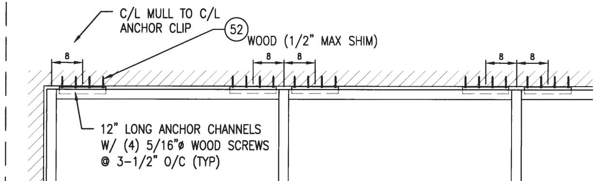
HEAD ANCHOR CONDITION A (CHANNEL)
