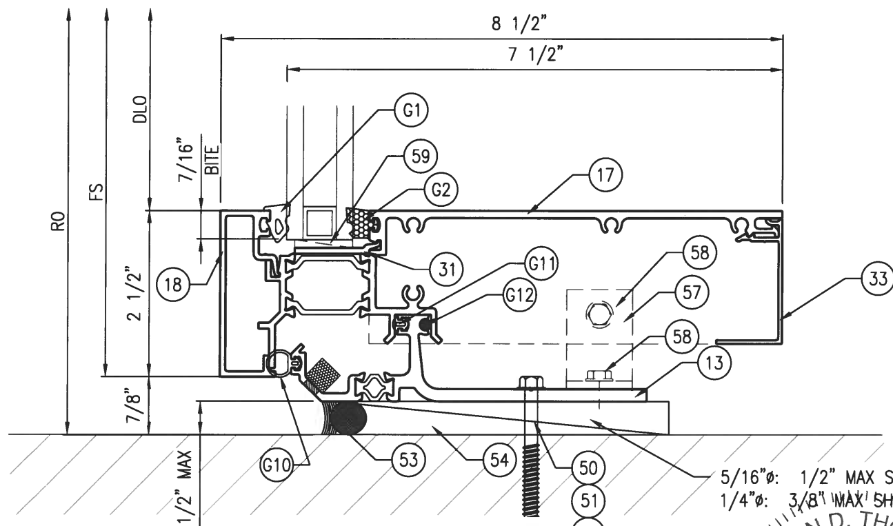
2 SUN 800T SILL CAPTURED Scale: 6" = 1'-0"
