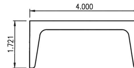
8 4 X 1.72 X.320 STR. ALUM CHANNEL HEAD ANCHOR Scale: 6" = 1'-0"
